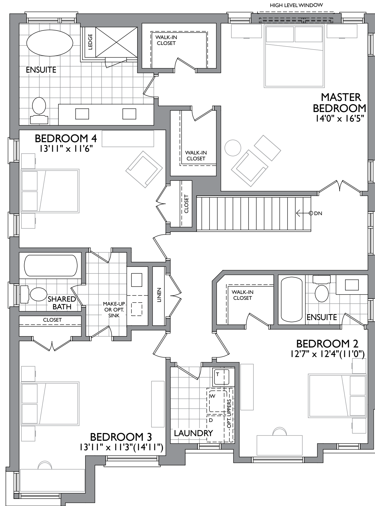
SECOND FLOOR ELEV. A
