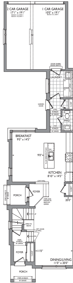
FIRST FLOOR BLOCK 116, 118 - 2 CAR BLOCK 121 - 1 CAR
