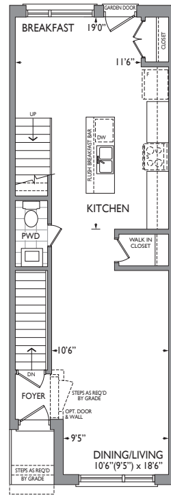
FIRST FLOOR ELEV. A, A1, B, B1
