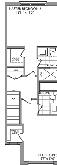
OPT. THIRD FLOOR - 3 BED/3BATH ELEV. A, A1, B, B1
