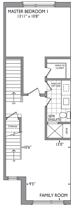
SECOND FLOOR ELEV. A, A1, B, B1
