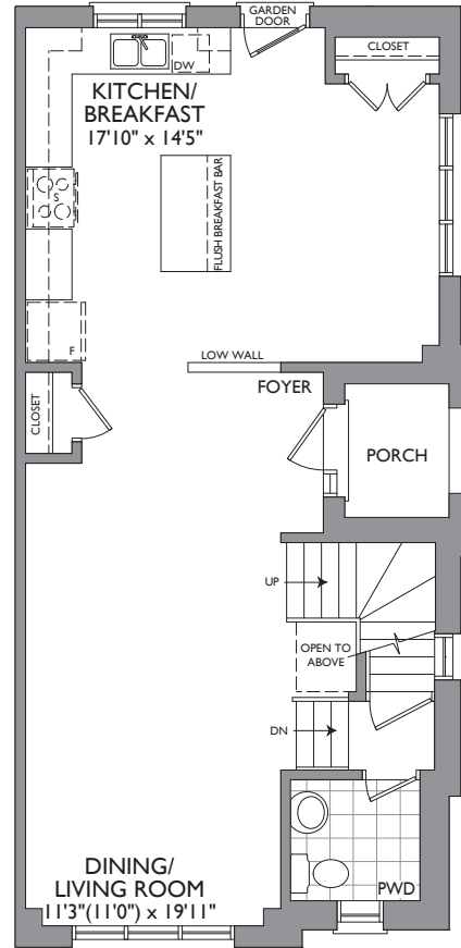
FIRST FLOOR ELEV. B 2 CAR - BLOCK 96, UNIT 1 ELEV. B ONLY
