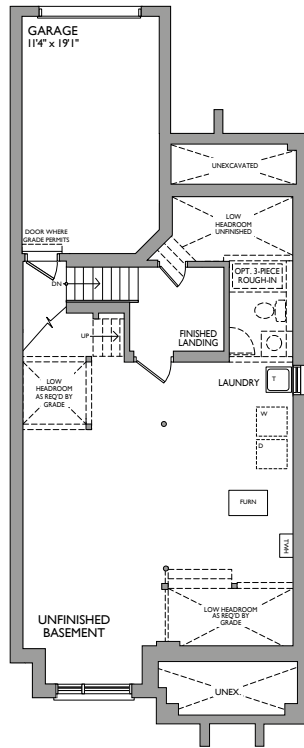
BASEMENT ELEVATION A
