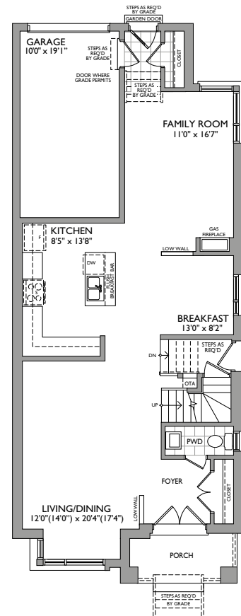
OPT. FIRST FLOOR ELEVATION A
