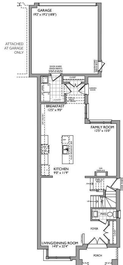
FIRST FLOOR ELEVATION A
