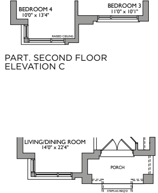
PART. FIRST FLOOR ELEVATION C
