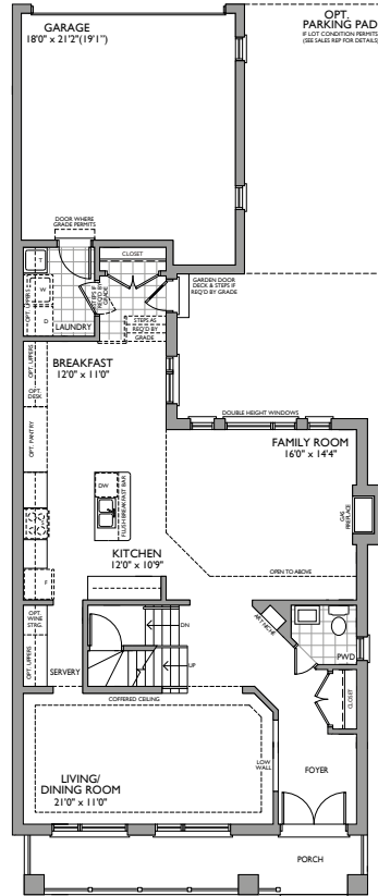
FIRST FLOOR ELEVATION A
