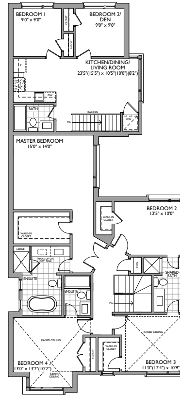
SECOND FLOOR ELEVATION A CORNER
