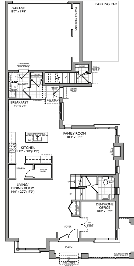
FIRST FLOOR ELEVATION A CORNER
