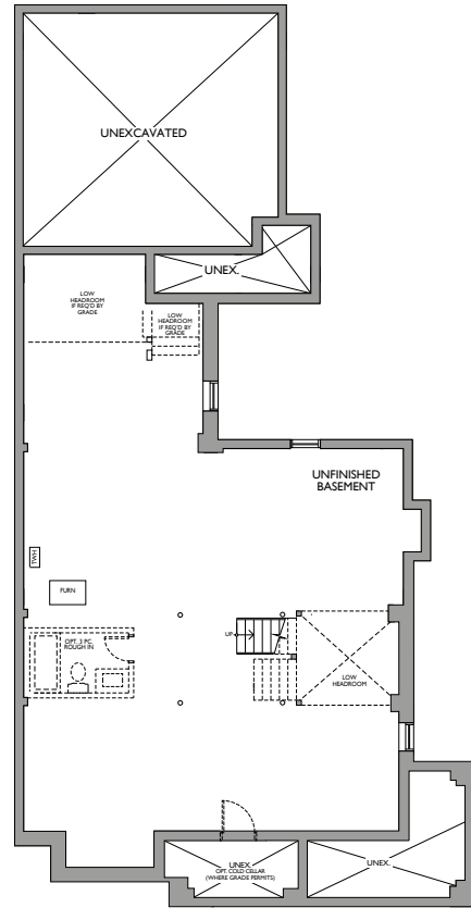
BASEMENT ELEVATION A CORNER
