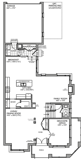
FIRST FLOOR ELEVATION B
