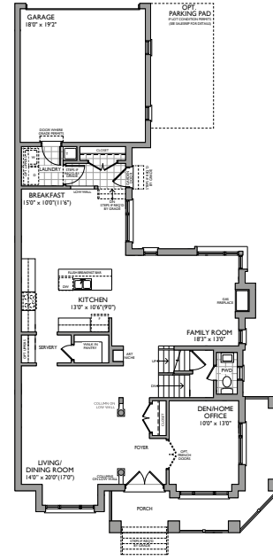
FIRST FLOOR ELEVATION A
