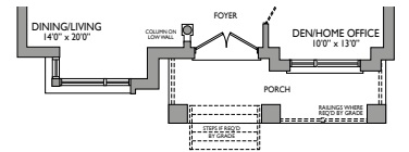
PART. FIRST FLOOR ELEVATION B
